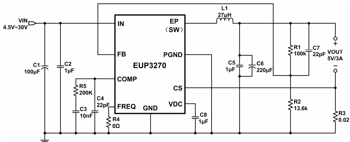
Figure 1. Application Circuit
